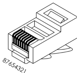
RJ45 Male connector
